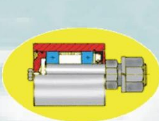
Carrier Roller
